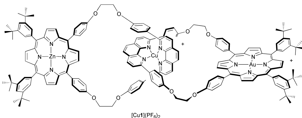
Fig. 2 Chemical structure of [\text{Cu1}](\text{PF}_6)_2 .
