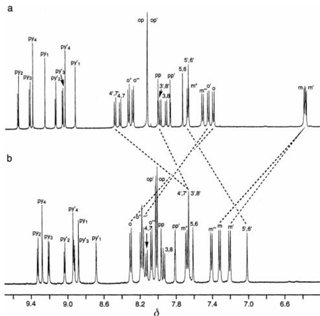
Fig. 7 ^1\text{H} -NMR spectra (500 MHz, \text{CD}_2\text{Cl}_2 ) of (a) [\text{CuI}](\text{PF}_6)_2 and (b) [1]\text{PF}_6 . Atom numbering as shown in Fig. 6.
