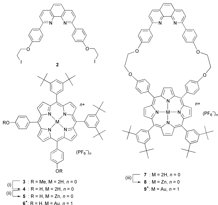
Fig. 4 Precursors to [2]-catenane [\text{CuI}](\text{PF}_6)_2 . (i) \text{BBr}_3 , \text{CH}_2\text{Cl}_2 , -78^\circ\text{C} , 100%; (ii) \text{Zn}(\text{OAc})_2 \cdot 2\text{H}_2\text{O} , \text{CHCl}_3/\text{CH}_3\text{OH} , reflux, 79%; (iii) same as (ii), 85%.
