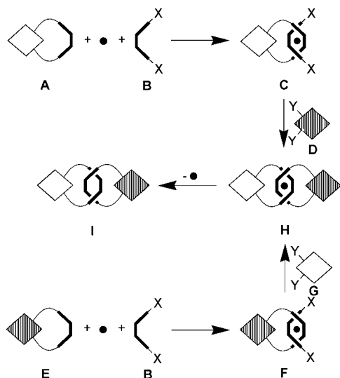
Fig. 3 Two strategies for the transition metal-templated synthesis of a [2]-catenane made with Zn and Au porphyrin-incorporating interlocked macrocycles. Symbols are as in Fig. 1. The black disk symbolises copper(i). See text for details.
