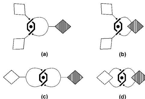
Fig. 1 Schematic representation of metal-complexed [2]-rotaxanes (a, b) and [2]-catenanes (c, d). The thick lines represent chelating fragments, the black disk is a metal cation, the open diamonds are Zn(II) porphyrins, and the hatched diamonds are Au(III) porphyrins.
