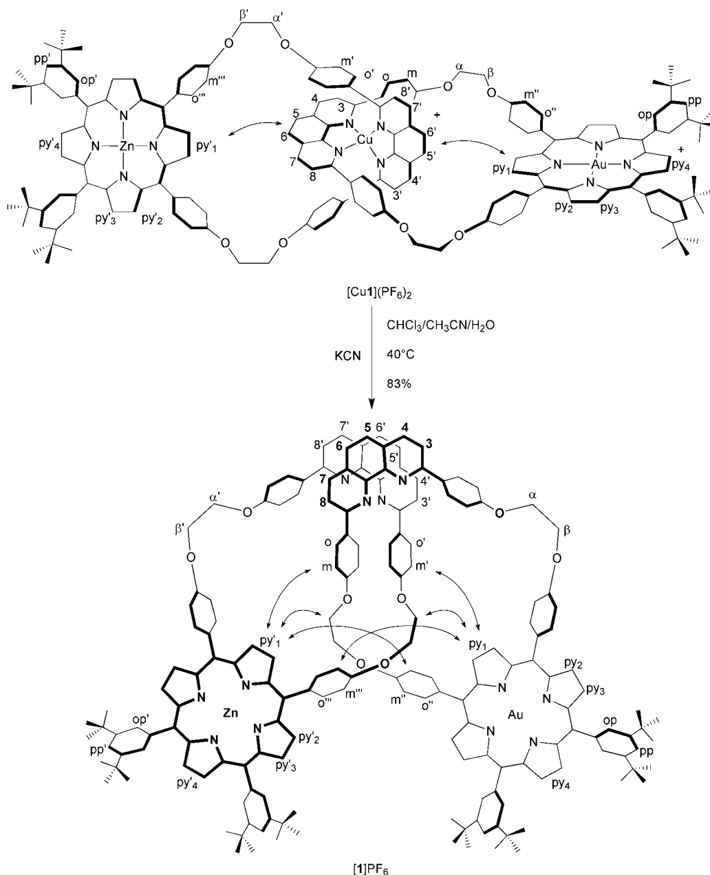
Fig. 6 Demetallation of [2]-catenane [\text{Cu}1](\text{PF}_6)_2 to [2]-catenane [\text{1}]\text{PF}_6 . Double bonds omitted for clarity. Double-headed arrows show selected ROESY correlations.
