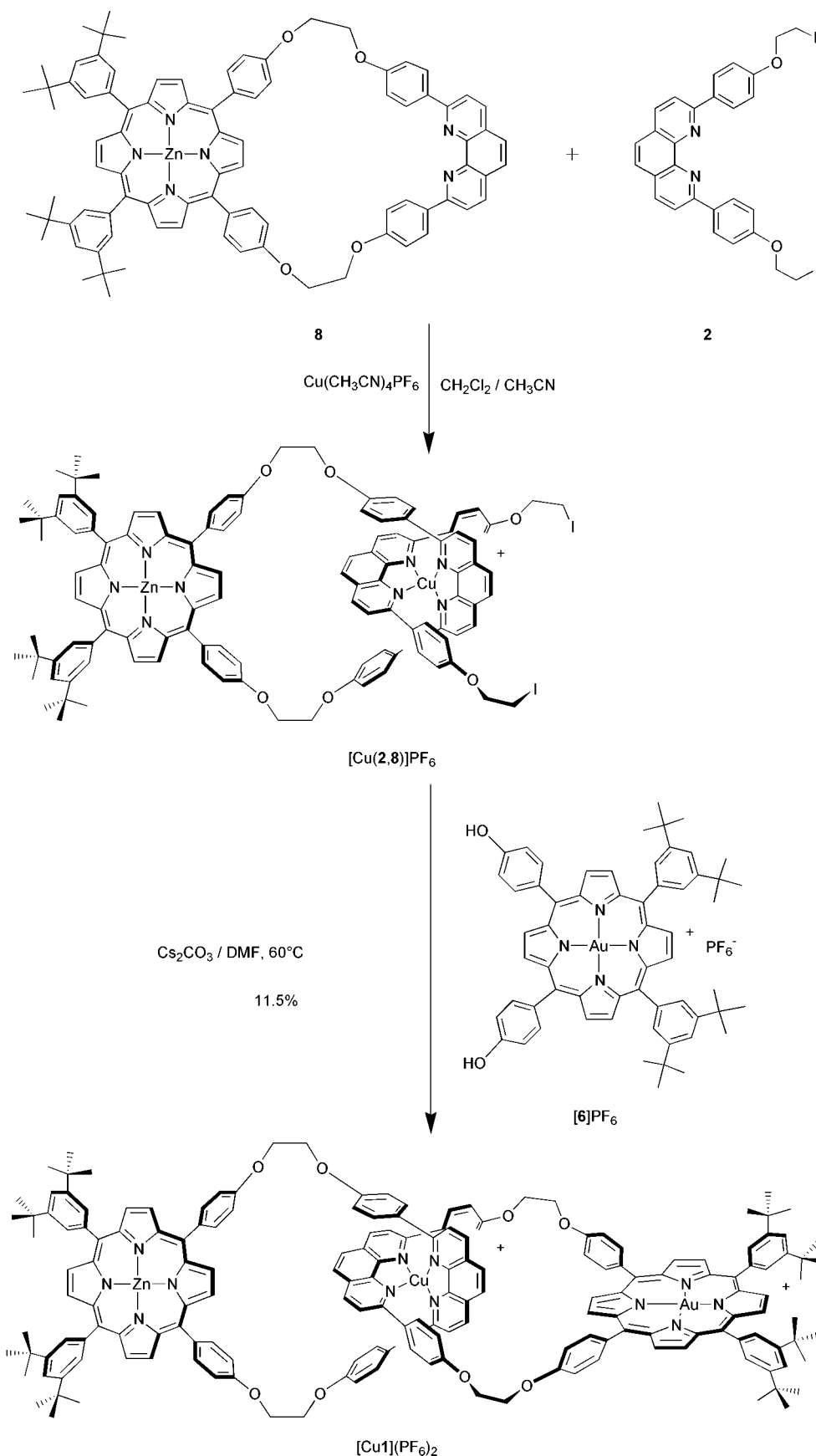
Fig. 5 Two-step preparation of Cu(I)-complexed [2]-catenate [\text{Cu}\mathbf{1}](\text{PF}_6)_2 .
